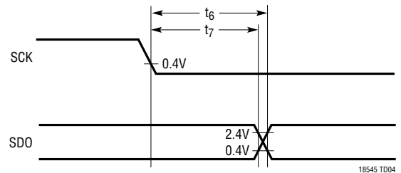
t_6 (Delay Time, \text{SCK} \downarrow to SDO Valid) t_7 (Time from Previous Data Remains Valid After \text{SCK} \downarrow )
