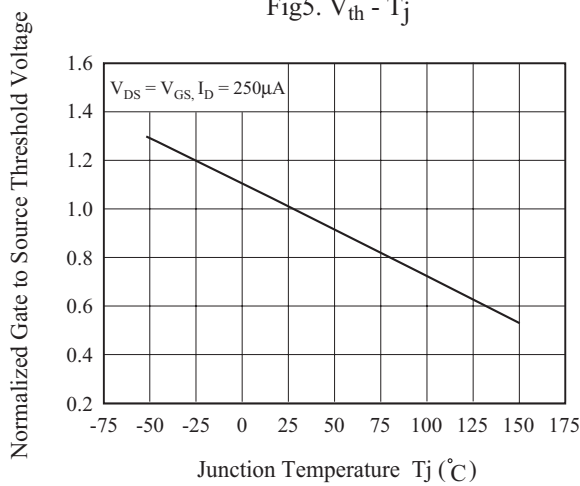
Fig5. V_{th} - T_J
