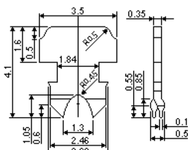
FOR SOLID WIRE 2 PRONGS CONTACTS
