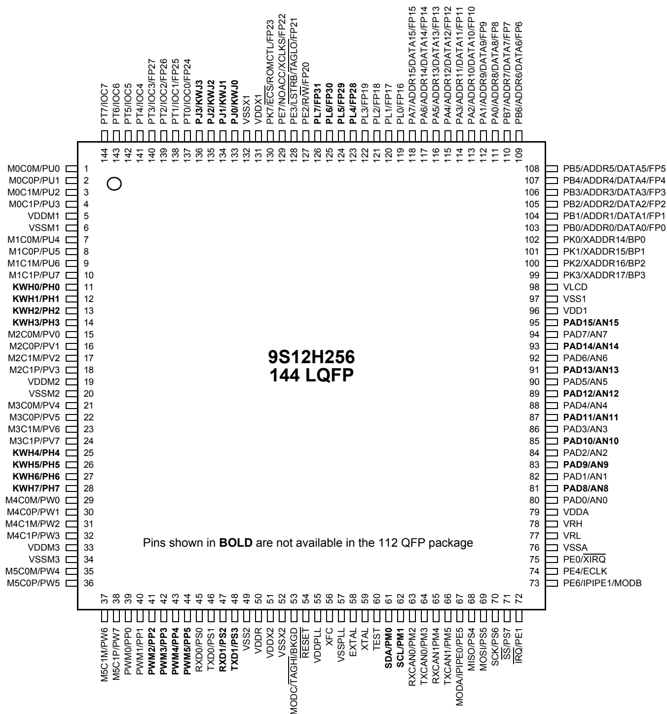
Figure 1. 144-Pin Package Signal Assignments for 9S12H256
