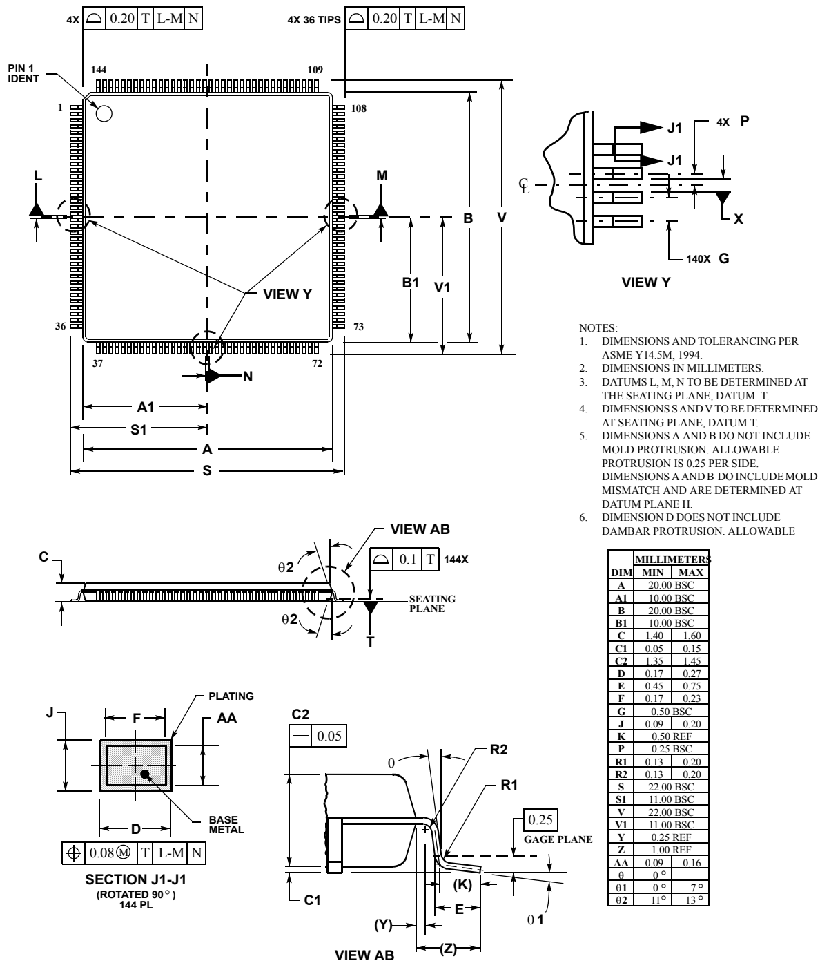
Figure 3. 144-pin LQFP Mechanical Dimensions (case no. 918-03)
