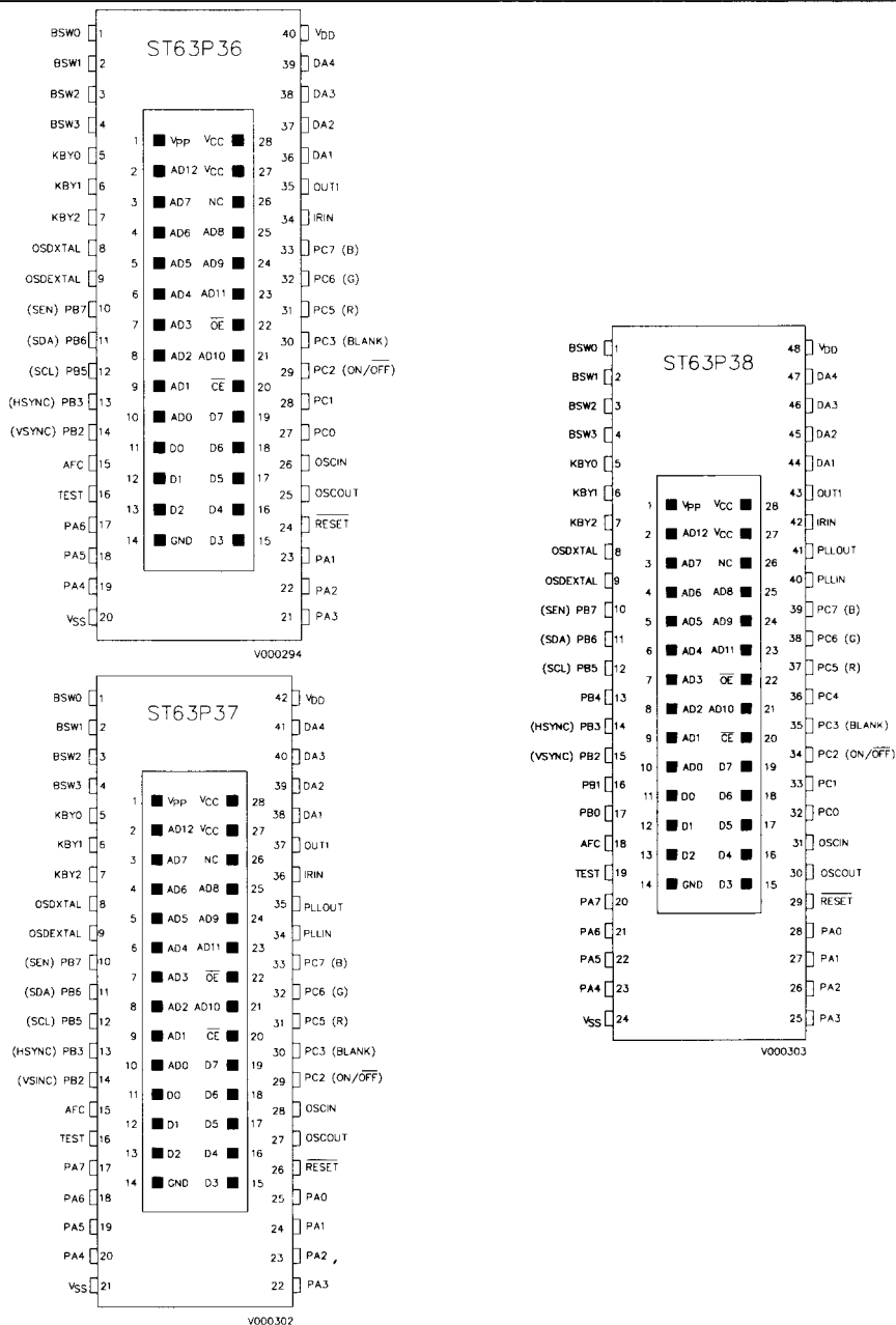
Figure 3 : ST63P36-ST63P37-ST63P38 Pin Configuration.
