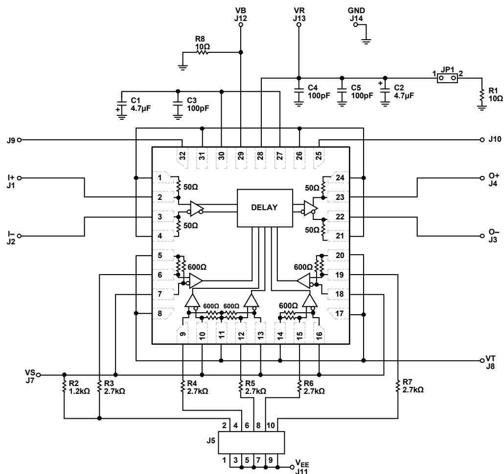
Figure 25. Typical Application Circuit
