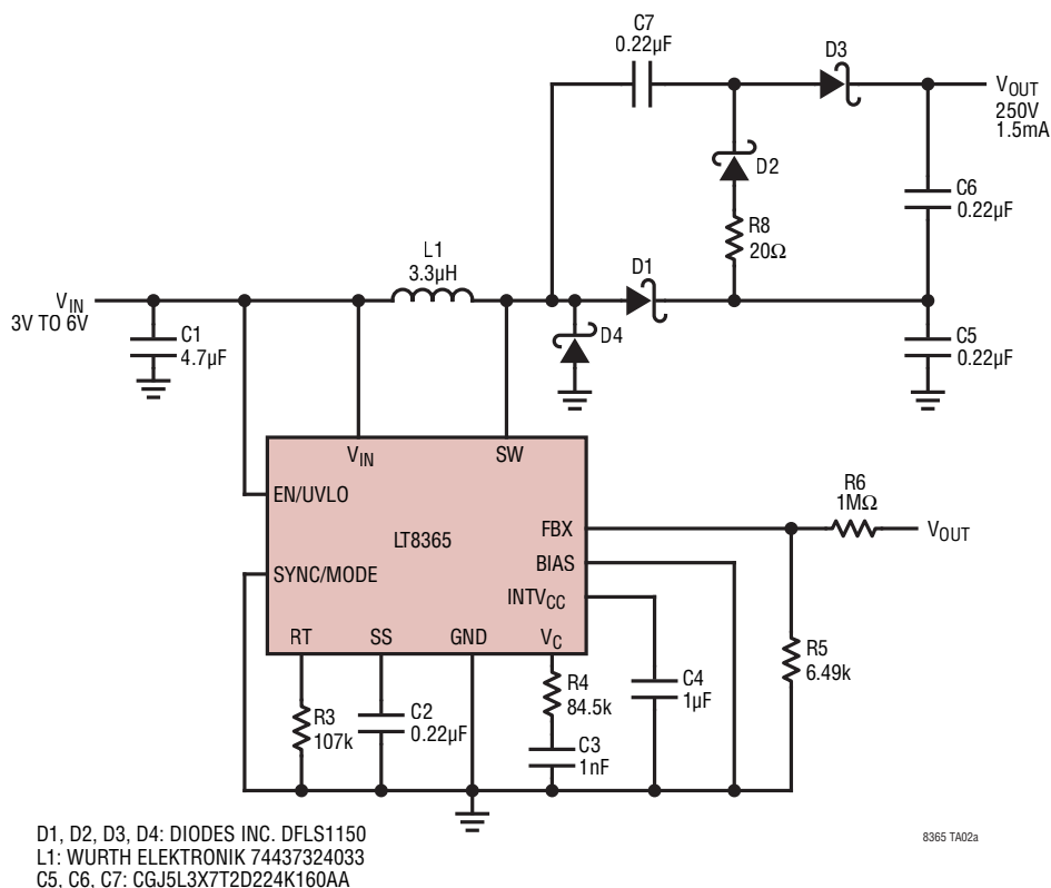
400kHz, 3V to 6V Input, 250V Output Boost Converter
