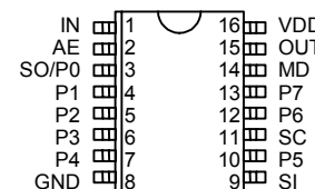
3D7418S SOL (300 Mil)
