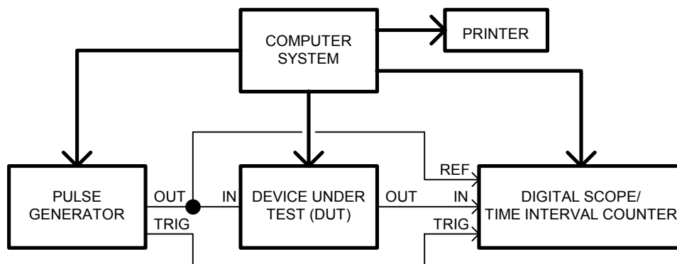
Figure 6: Test Setup
