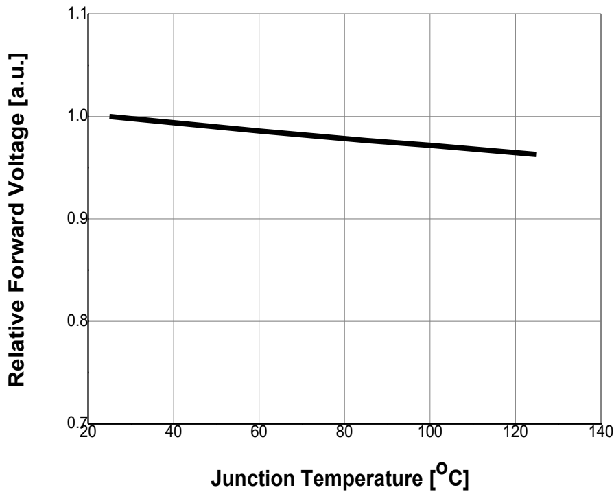
Fig 7. Relative Forward Voltage vs. Junction Temperature, I_F=180\text{mA}
