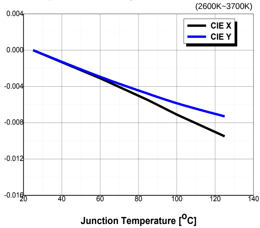
Fig 8. Junction Temp. vs. CIE X, Y Shift, I_F=180\text{mA}
