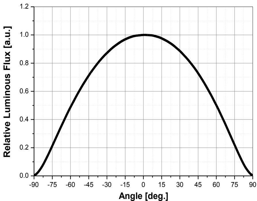
Fig 2. Radiant pattern, T_j=25^{\circ}\text{C} , I_F=180\text{mA}
