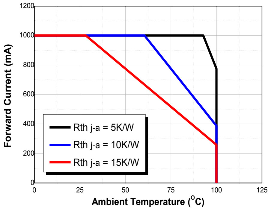
Fig 9. Maximum Forward Current vs. Ambient Temperature, T_j(\text{max.})=125^{\circ}\text{C} , I_F=1000\text{mA}
