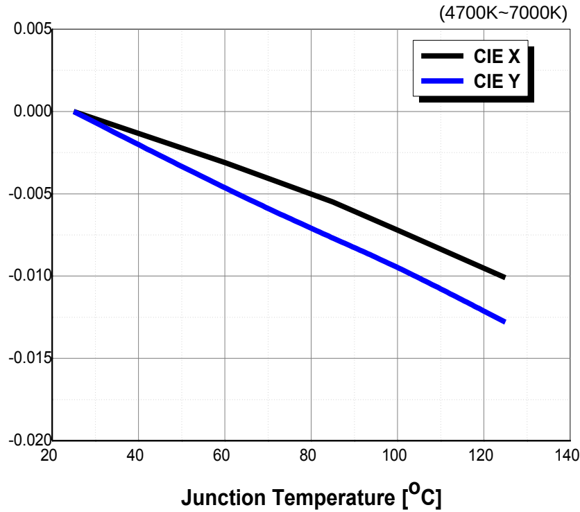
Fig 8. Junction Temp. vs. CIE X, Y Shift, I_F=180\text{mA}
