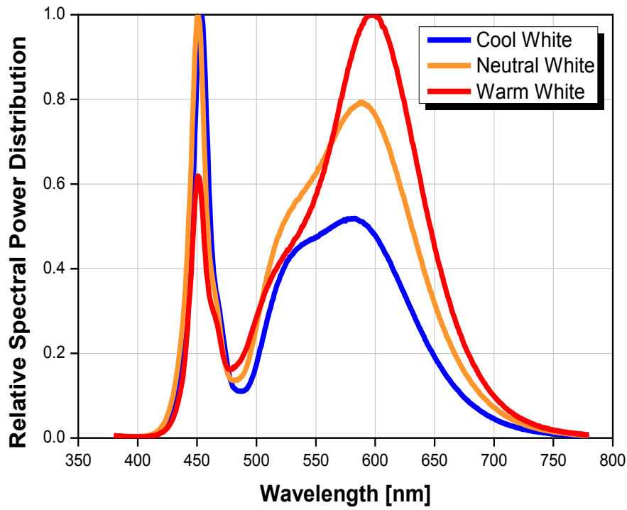
Fig 1. Color Spectrum, T_j=25^{\circ}\text{C} , I_F=180\text{mA}
