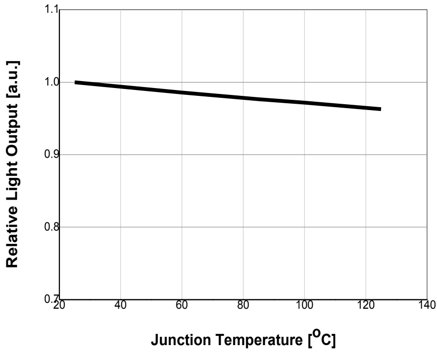
Fig 6. Relative Light Output vs. Junction Temperature, I_F=180\text{mA}
