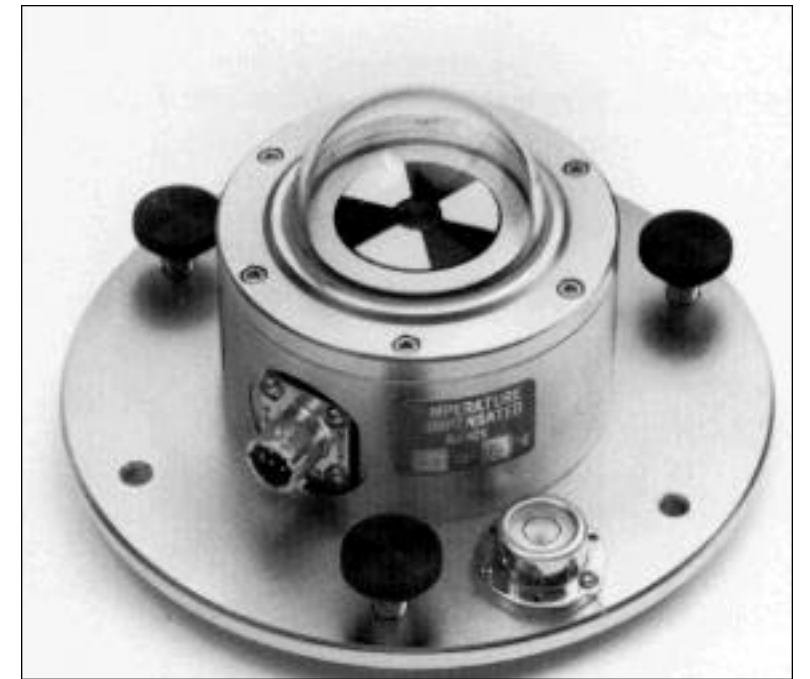
The Model 095 Pyranometer
