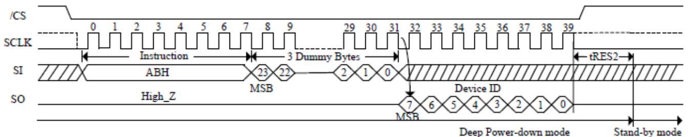
Figure 12. Release Power-Down/Read Device ID Sequence Diagram
