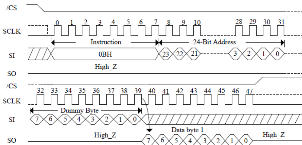
Figure 6. Fast Read Sequence Diagram
