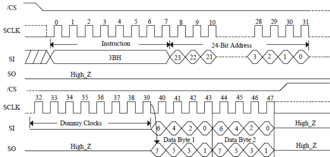
Figure 7. Dual Output Fast Read Sequence Diagram
