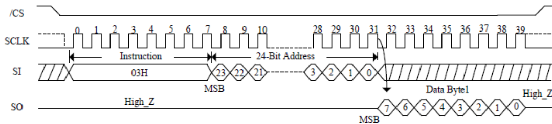
Figure 5. Read Data Bytes Sequence Diagram
