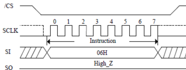
Figure 1. Write Enable Sequence Diagram
