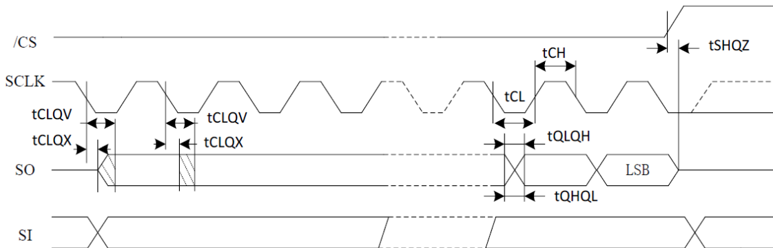
Figure 22. Output Timing
