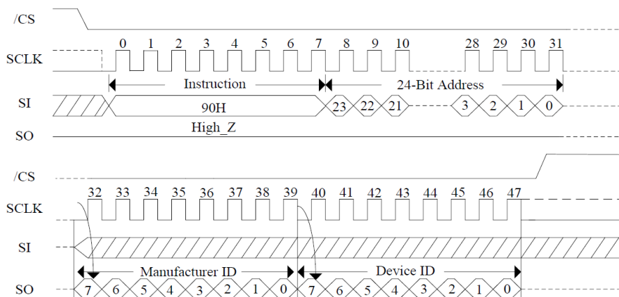
Figure 8. Read Manufacture ID/ Device ID Sequence Diagram
