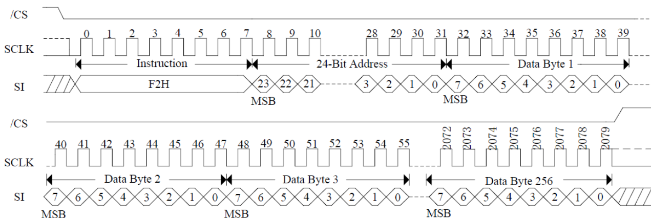
Figure 14. Page Program Sequence Diagram
