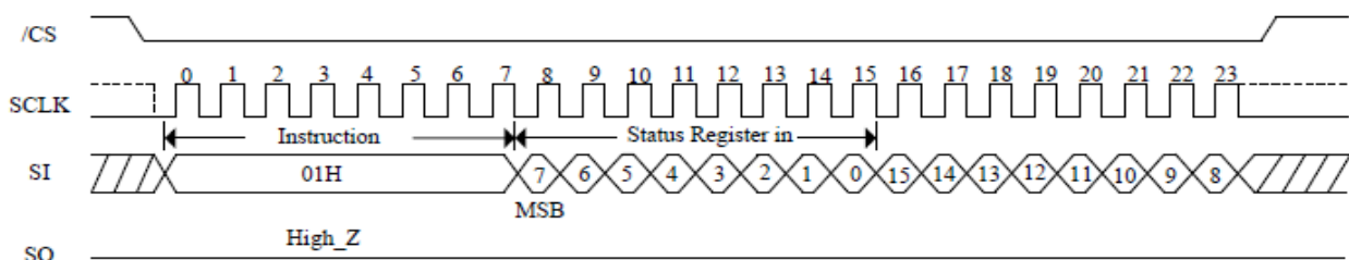
Figure 4. Write Status Register Sequence Diagram
