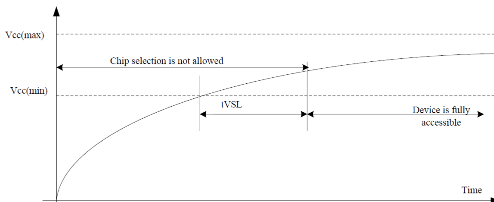
Figure 19. Power-up Timing and Voltage Levels
