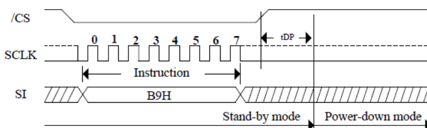
Figure 10. Deep Power-Down Sequence Diagram
