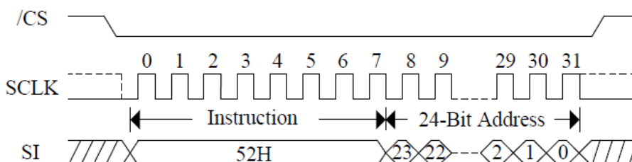
Figure 16. 32KB Block Erase Sequence Diagram
