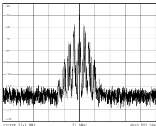
Figure 10. RF Frequency = 98.1 MHz, Frequency Deviation = 10.5 kHz, Modulation Frequency = 15 kHz, Pre-emphasis OFF
