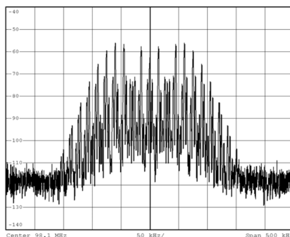
Figure 11. RF Frequency = 98.1 MHz, Frequency Deviation = 10.5 kHz, Modulation Frequency = 15 kHz, Pre-emphasis = 75 \mu s
