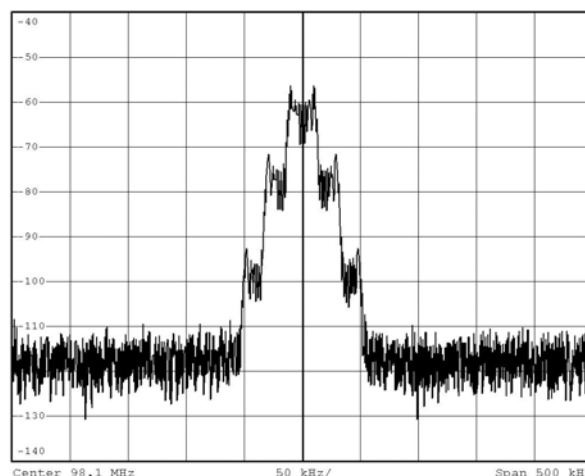
Figure 9. RF Frequency = 98.1 MHz, Frequency Deviation = 10.5 kHz, Modulation Frequency = 1 kHz, Pre-emphasis = 75 \mu s
