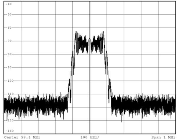
Figure 13. RF Frequency = 98.1 MHz, Frequency Deviation = 75 kHz, Modulation Frequency = 1 kHz, Pre-emphasis = 75 µs
