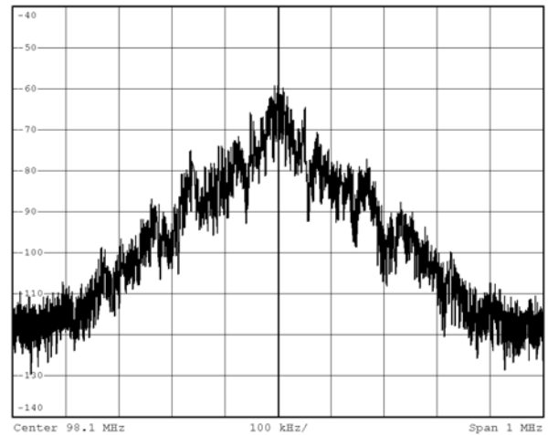
Figure 15. RF Frequency = 98.1 MHz, Frequency Deviation = 75 kHz, Modulation Frequency = 15 kHz, Pre-emphasis = 75 µs
