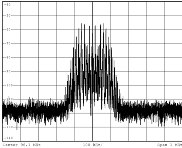
Figure 14. RF Frequency = 98.1 MHz, Frequency Deviation = 75 kHz, Modulation Frequency = 15 kHz, Pre-emphasis OFF
