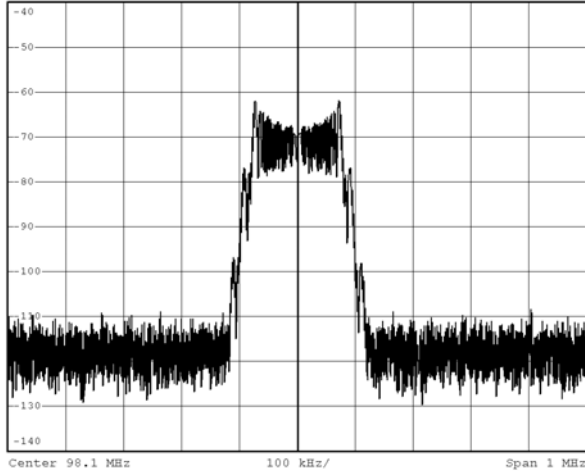
Figure 12. RF Frequency = 98.1 MHz, Frequency Deviation = 75 kHz, Modulation Frequency = 1 kHz, Pre-emphasis OFF
