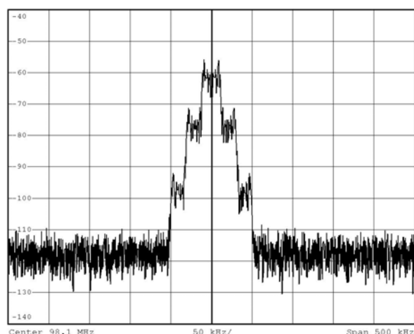
Figure 8. RF Frequency = 98.1 MHz, Frequency Deviation = 10.5 kHz, Modulation Frequency = 1 kHz, Pre-emphasis OFF
