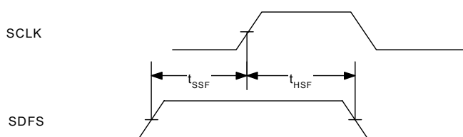
Figure xx. SDFS Timing Requirements (SBM=0)
