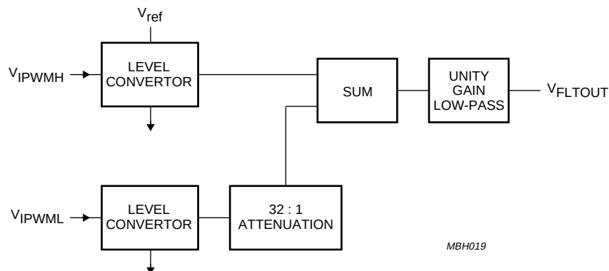
Fig.5 Block diagram of the VCM driver PWM filter.
