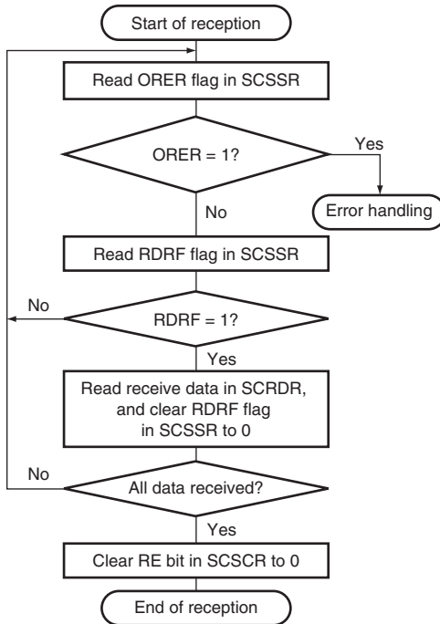
Figure 14.12 Sample Flowchart for Receiving Serial Data (1)
