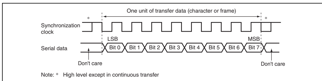
Figure 14.8 Data Format in Clock Synchronous Communication
