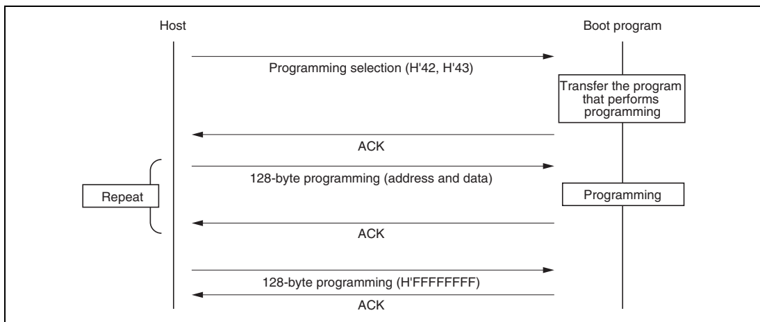
Figure 19.25 Sequence of Programming
