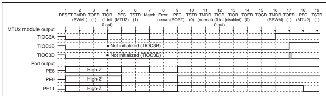
Figure 10.147 Error Occurrence in PWM Mode 1, Recovery in Reset-Synchronized PWM Mode
