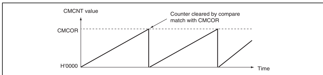
Figure 16.2 Counter Operation
