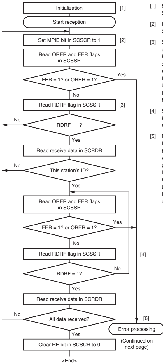
Figure 14.18 Sample Multiprocessor Serial Reception Flowchart (1)
