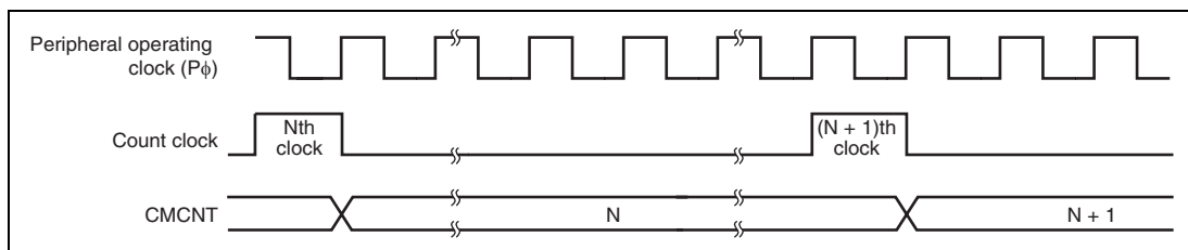
Figure 16.3 Count Timing
