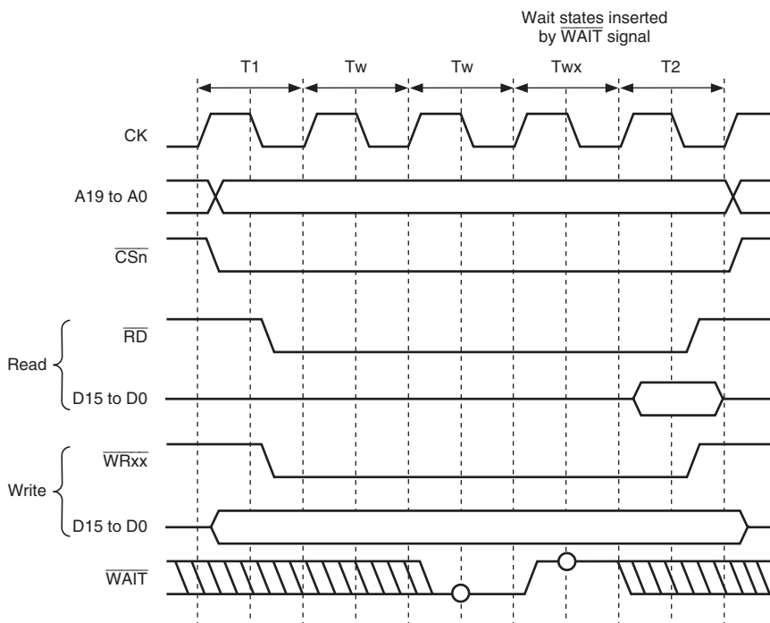
Figure 9.8 Wait State Timing for Normal Space Access (Wait State Insertion Using \overline{\text{WAIT}} Signal)
