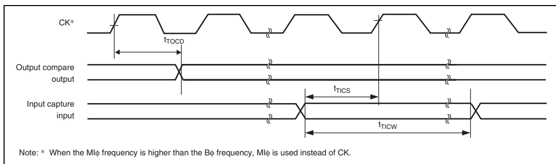
Figure 24.18 MTU2S Input/Output Timing
