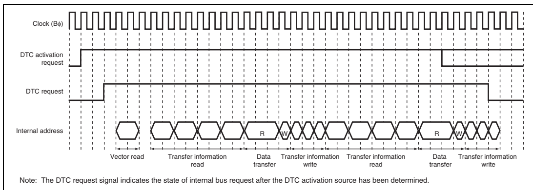
Figure 8.12 Example of DTC Operation Timing: Chain Transfer (Activated by On-Chip Peripheral Module; Iφ: Bφ: Pφ=1: 1/2: 1/2; Data Transferred from On-Chip Peripheral Module to On-Chip RAM; Transfer Information is Written in 3 Cycles)
