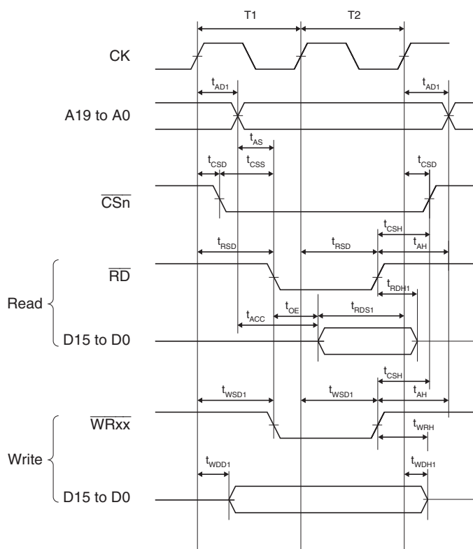
Figure 24.11 Basic Bus Timing for Normal Space (No Wait)
