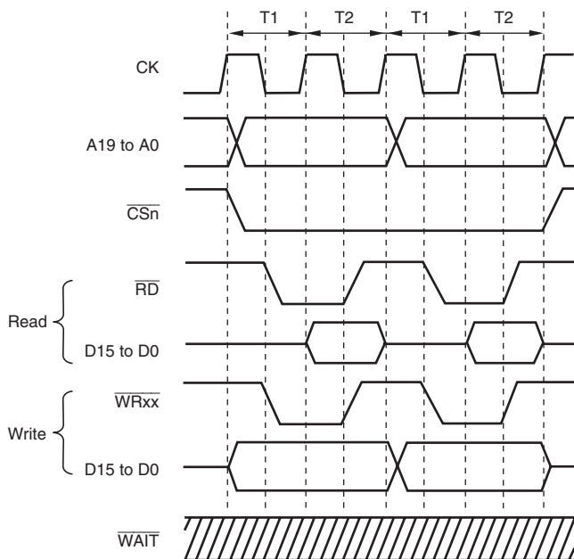
Figure 9.4 Continuous Access for Normal Space 2 Bus Width = 16 Bits, Longword Access, WM Bit in CSnWCR = 1 (Access Wait = 0, Cycle Wait = 0)
