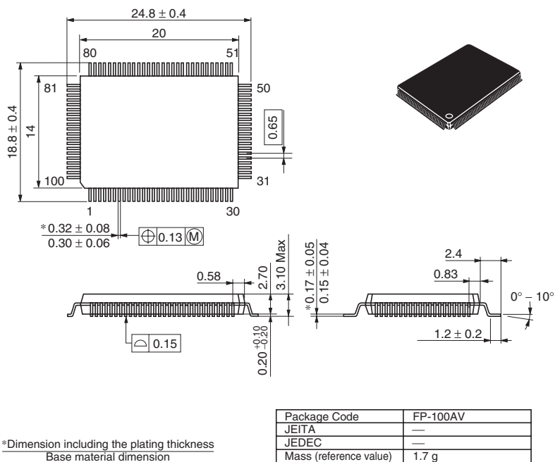
Figure D.3 FP-100AV
