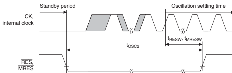
Figure 24.3 Power-On Oscillation Settling Timing
