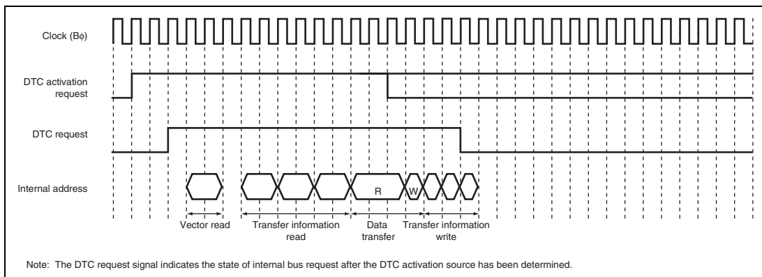
Figure 8.13 Example of DTC Operation Timing: Normal or Repeat Transfer in Short Address Mode (Activated by On-Chip Peripheral Module; Iφ: Bφ: Pφ=1: 1/2: 1/2; Data Transferred from On-Chip Peripheral Module to On-Chip RAM; Transfer Information is Written in 3 Cycles)
