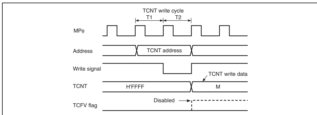
Figure 10.135 Contention between TCNT Write and Overflow
