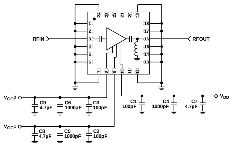
Figure 22. Typical Application Circuit
