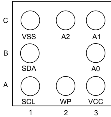
Fig.3 BU9880GUL-W(bottom view)
