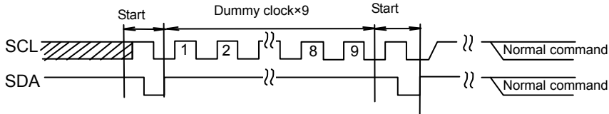
Fig.39-(b) The case of START+9 Dummy clock + START + command input
