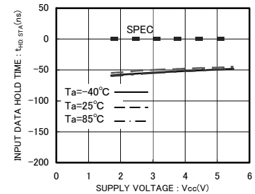
Fig.18 Input Data Hold Time t_{HD:DAT(HIGH)}
