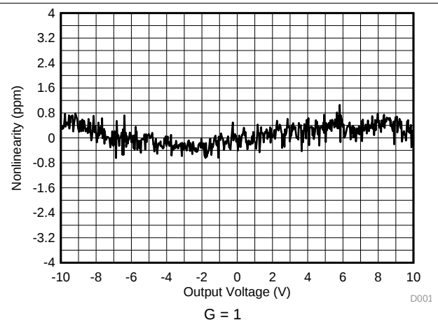
Figure 42. Gain Nonlinearity
