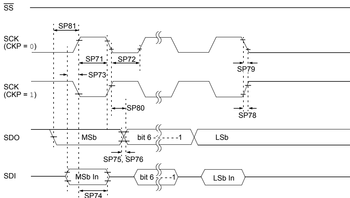
FIGURE 25-14: SPI MASTER MODE TIMING (CKE = 1, SMP = 1)
