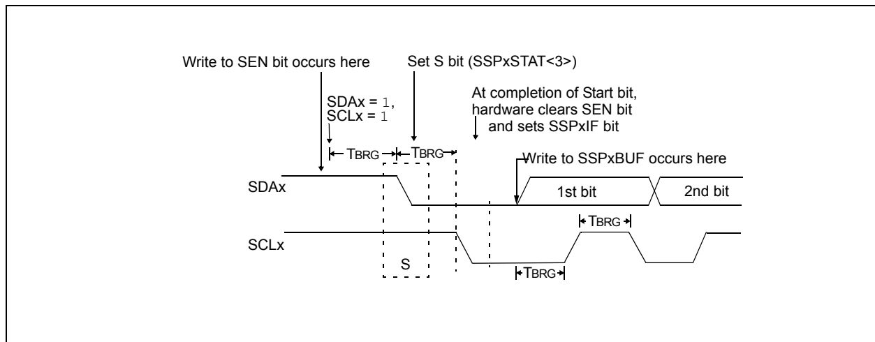
FIGURE 20-26: FIRST START BIT TIMING
