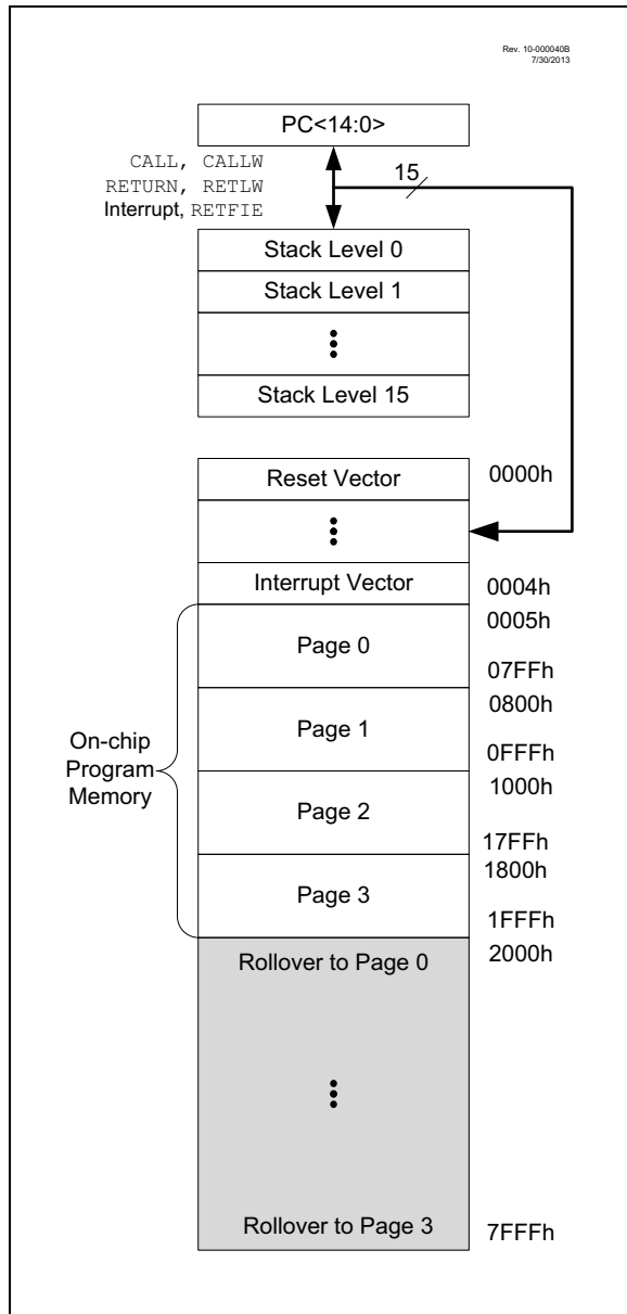
FIGURE 3-1: PROGRAM MEMORY MAP AND STACK FOR PIC16LF1566/1567
