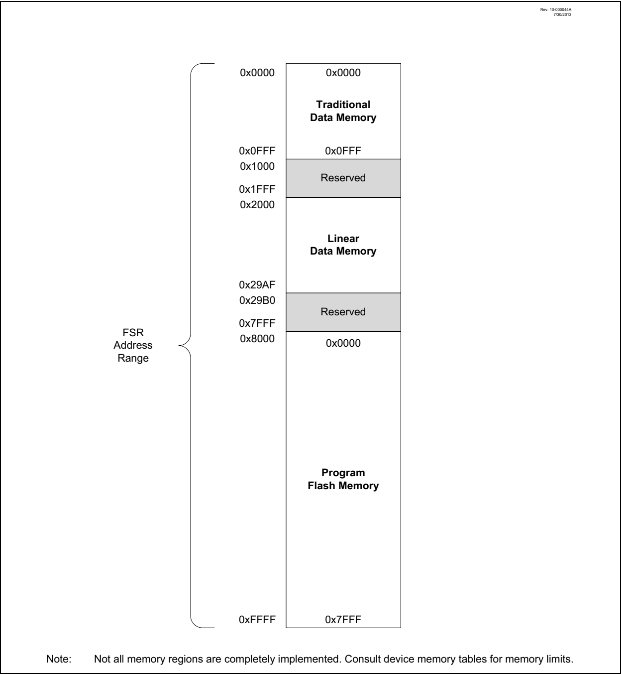
FIGURE 3-8: INDIRECT ADDRESSING
