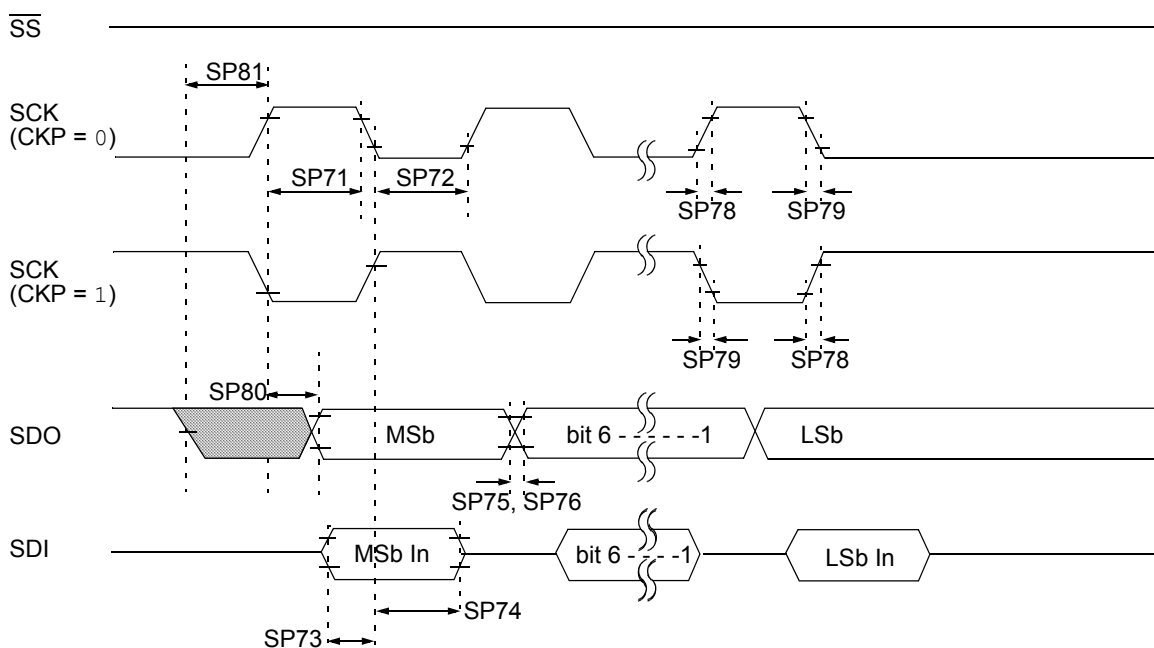
FIGURE 25-13: SPI MASTER MODE TIMING (CKE = 0, SMP = 0)
