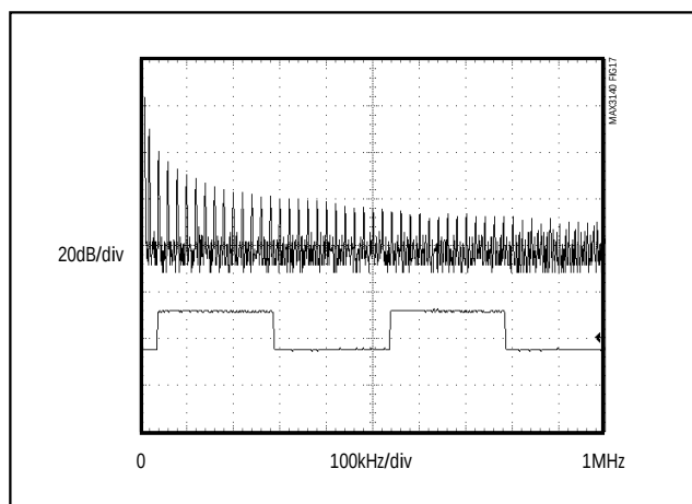
Figure 17. Driver Output Waveform and FFT Plot of MAX3140 with \text{SRL} = \text{GND} , Transmitting at 20kHz
