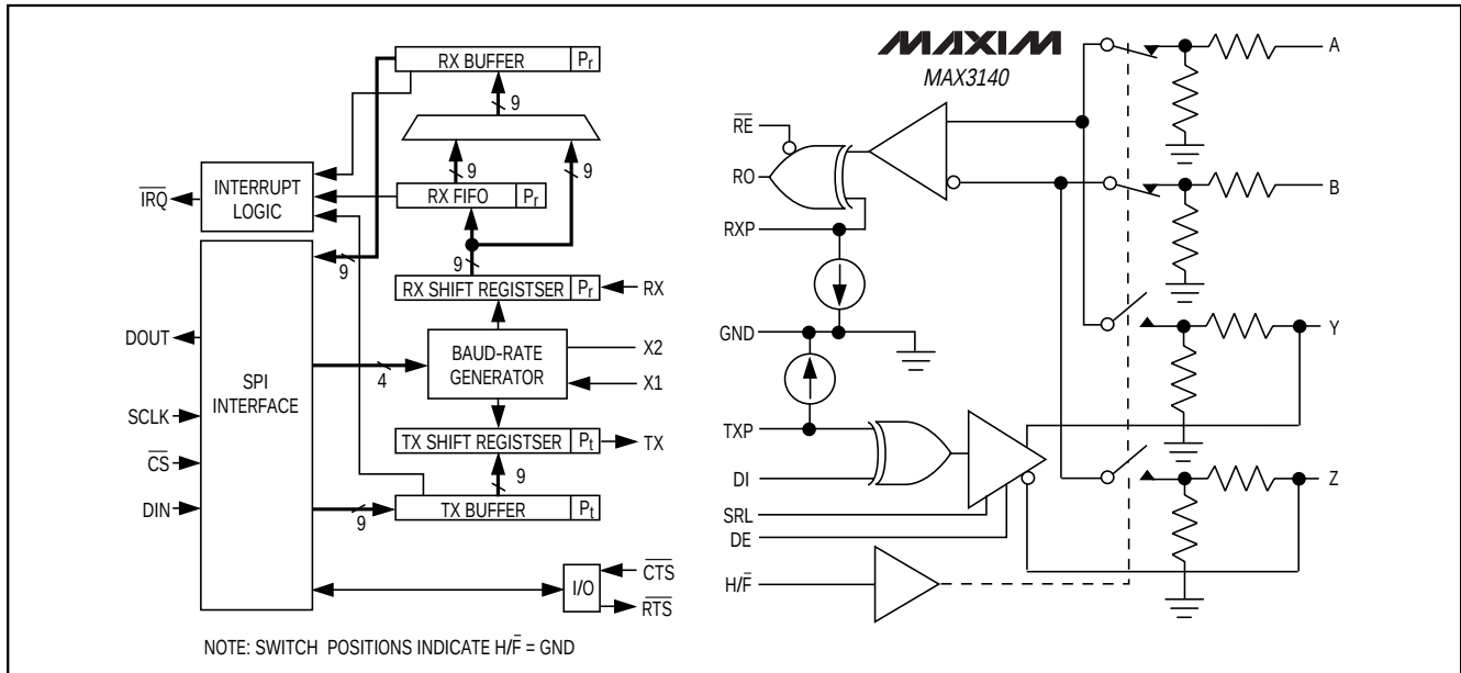
Figure 10. Functional Diagram
