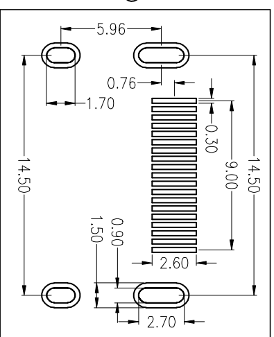
RECOMMENDED P.C.B HOLE LAYOUT COMPONENT SIDE VIEW(TOLERANCE: +/-0.05)
