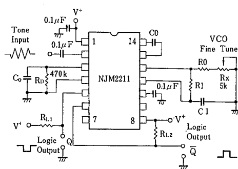
Figure 4. Tone Detection
