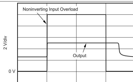
Figure 20. Noninverting Differential Input Overload
