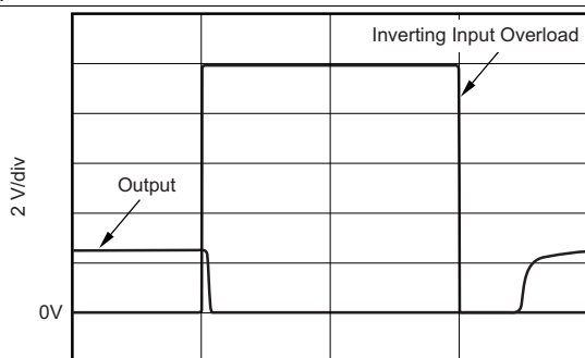
Figure 19. Inverting Differential Input Overload
