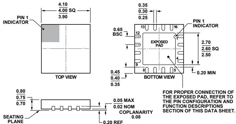
Figure 35. 16-Lead Lead Frame Chip Scale Package [LFCSP] 4 mm × 4 mm Body and 0.75 mm Package Height (CP-16-17) Dimensions shown in millimeters
