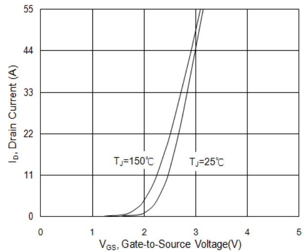
Fig.8: Transfer Characteristics
