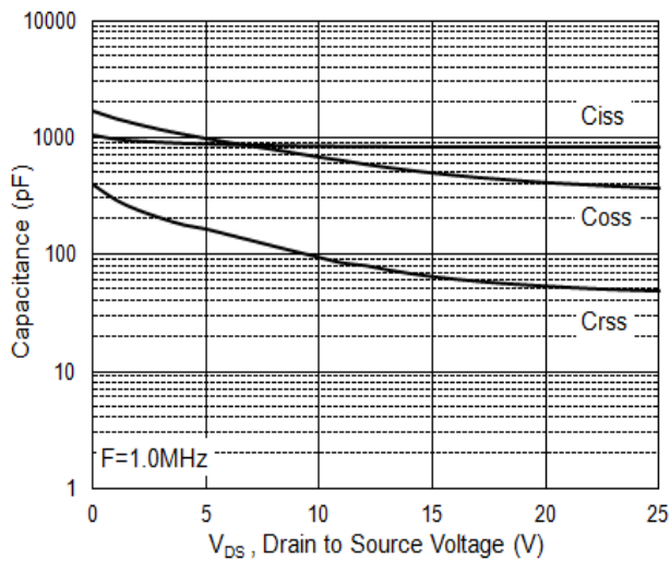
Fig.9: Capacitance
