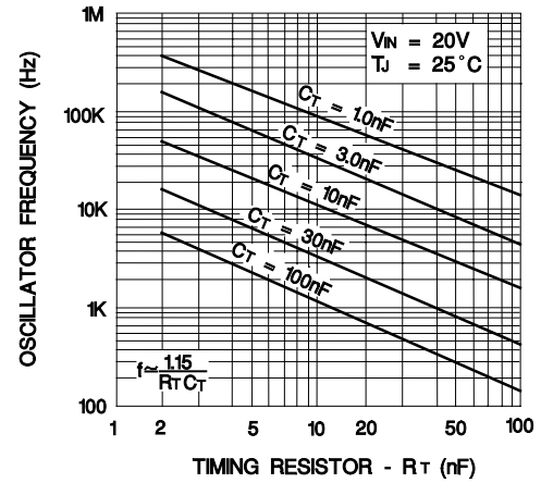
Oscillator Frequency vs Timing Components
