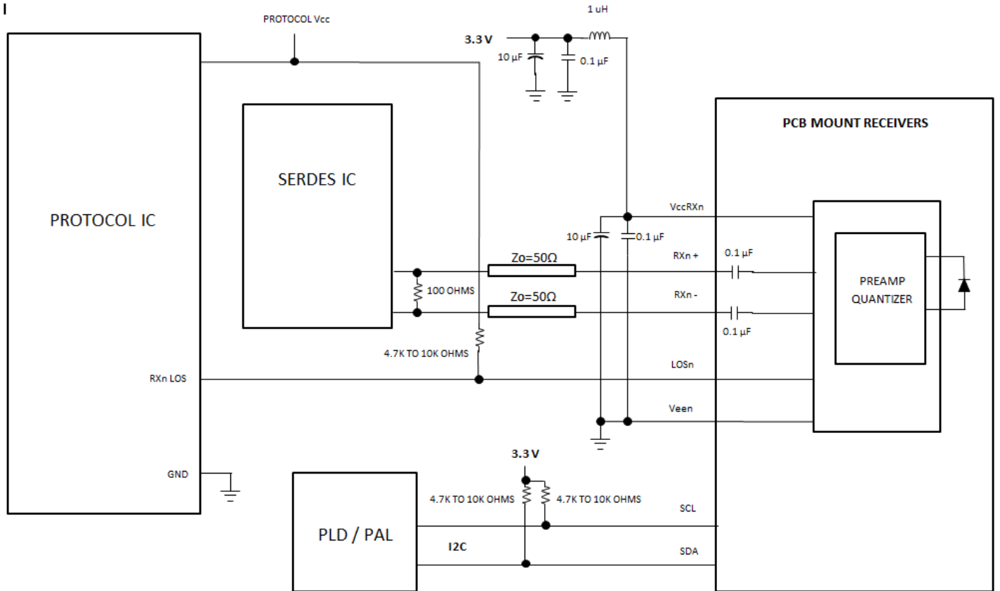
FIGURE 3 RECOMMENDED PCB MOUNT DUAL-RECEIVER HOST BOARD SCHEMATIC SINGLE RECEIVER SHOWN (2X RECEIVERS PER MODULE)
