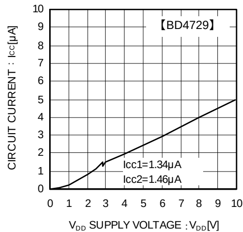
Fig.2 Circuit Current
