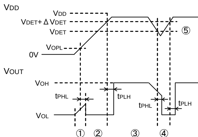
Fig.11 Timing Waveform
