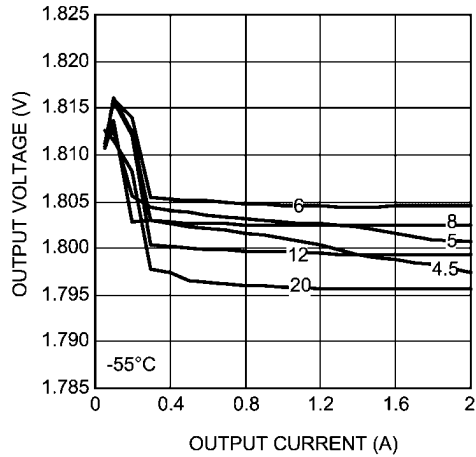
Line and Load Regulation @ -55°C
