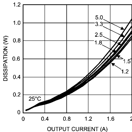
Dissipation 6V Input @ 25°C
