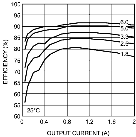
Efficiency 20V Input @ 25°C
