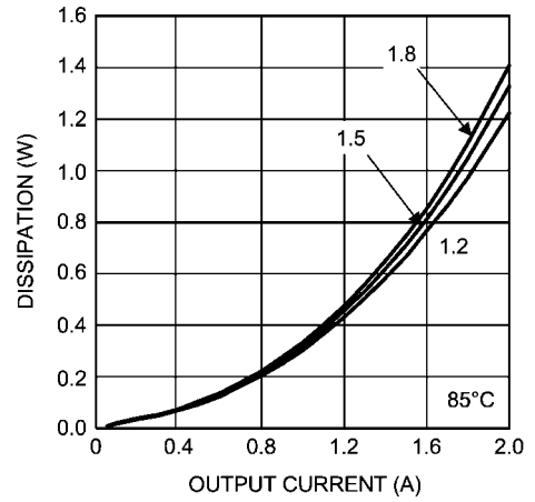
Dissipation 4.5V Input @ 85°C
