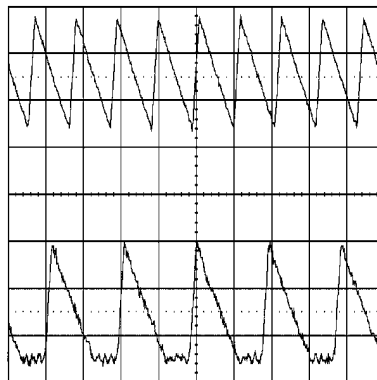
CCM and DCM Operating Modes V IN = 12V, V O = 3.3V, I O = 2A/0.26A 2 μsec/div
