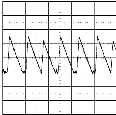
Transition Mode Operation V_{IN} = 12V, V_O = 3.3V, I_O = 0.29A 2 \mu\text{sec/div}
