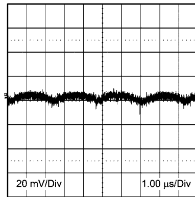
Output Ripple 12V IN 3.3V O 2A 20mV/div 1μSec/div
