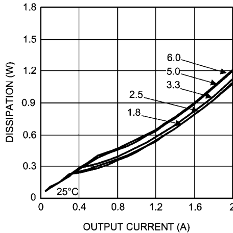
Dissipation 20V Input @ 25°C
