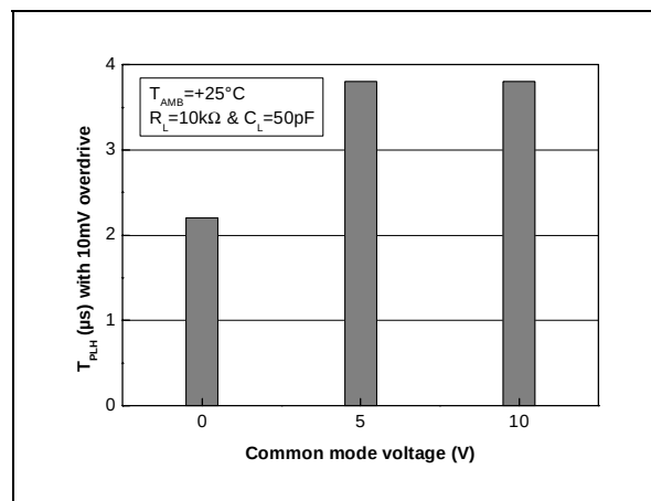
T_{PLH} vs V_{ICM} @ V_{CC}=5V and 10mV overdrive
