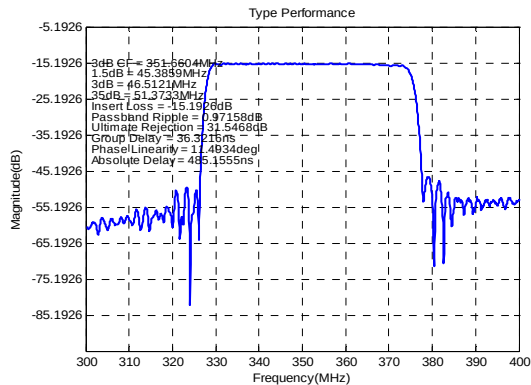
Frequency Response
