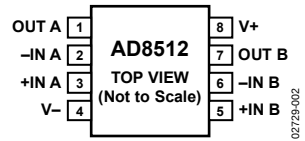
Figure 4. 8-Lead SOIC_N (R Suffix)
