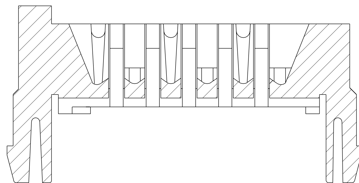
SECTION "E"-"E"
