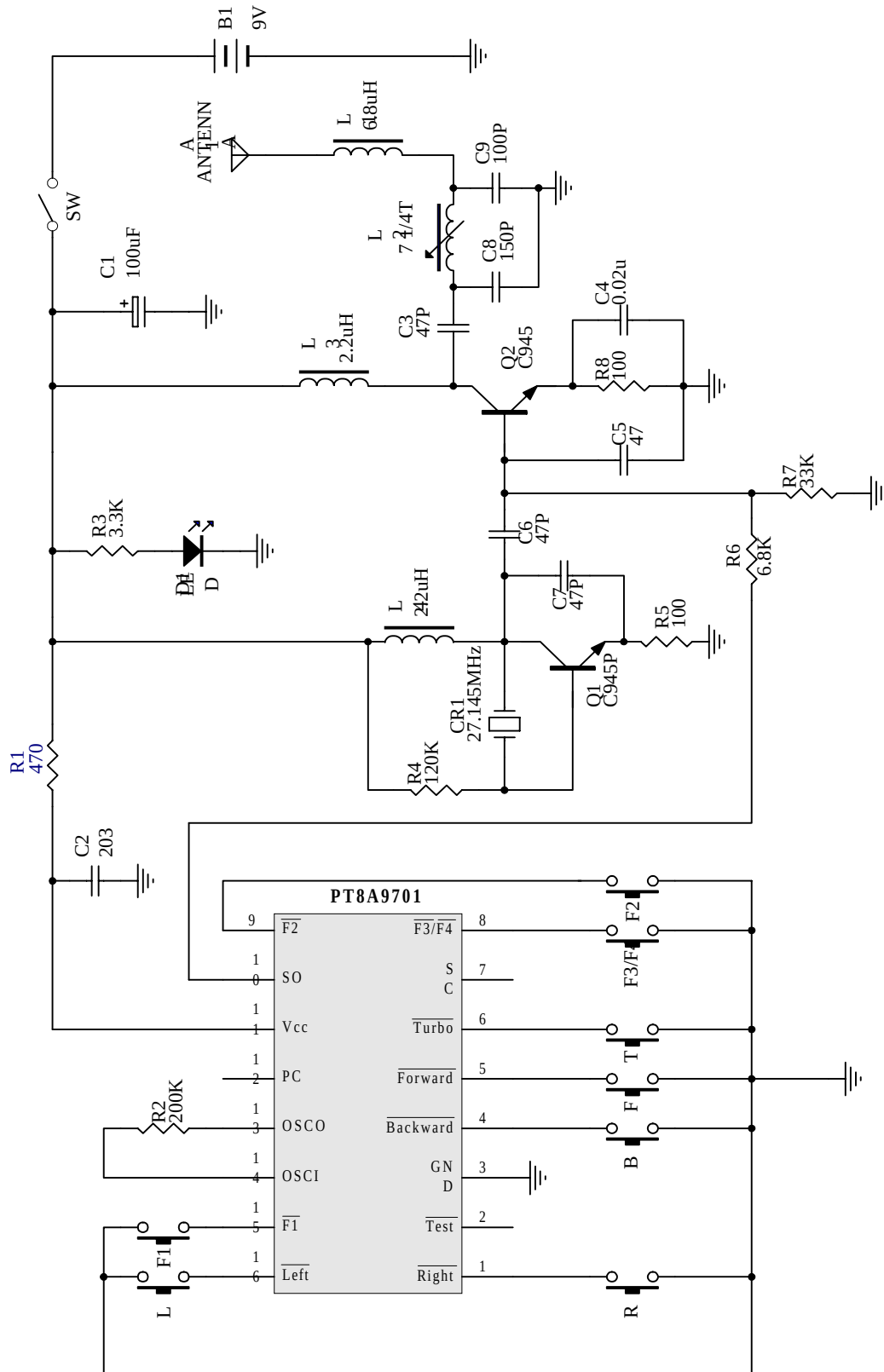
Figure 5. Typical Application Circuit of PT8A9701
