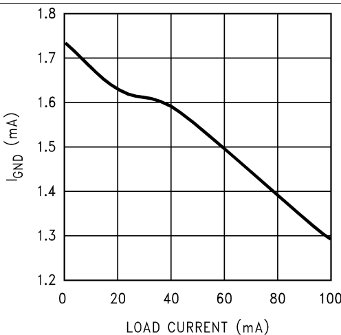
Figure 5. Ground Pin Current vs Load Current
