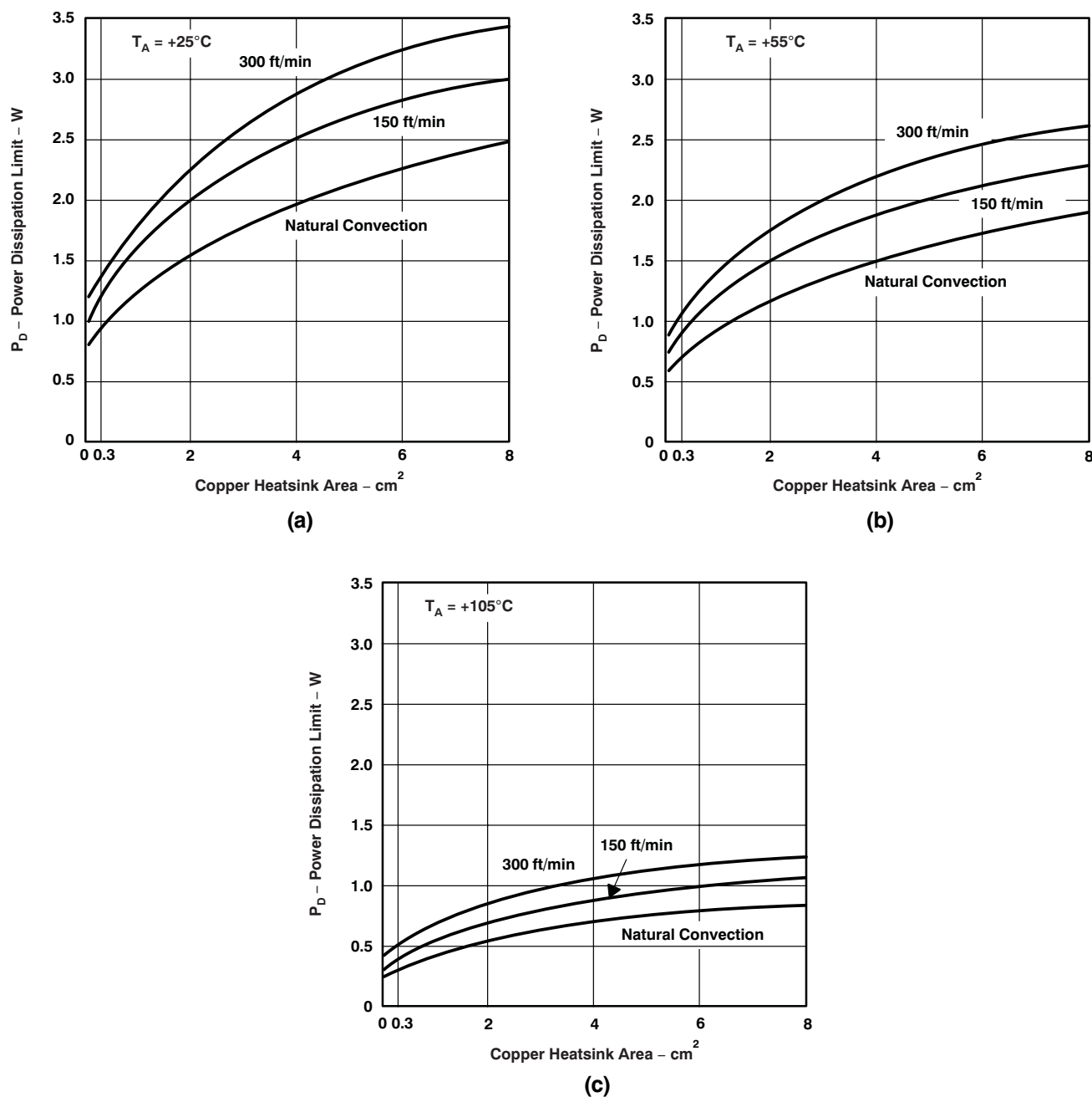
Figure 28. Power Ratings of the PWP Package at Ambient Temperatures of +25°C, +55°C, and +105°C
