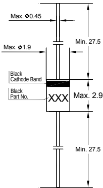
Glass Case DO-34 Dimensions in mm
