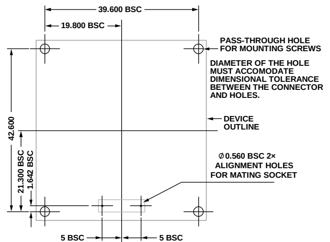
Figure 26. Mounting Example
