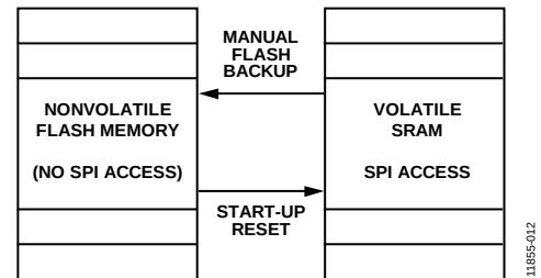
Figure 15. SRAM and Flash Memory Diagram
