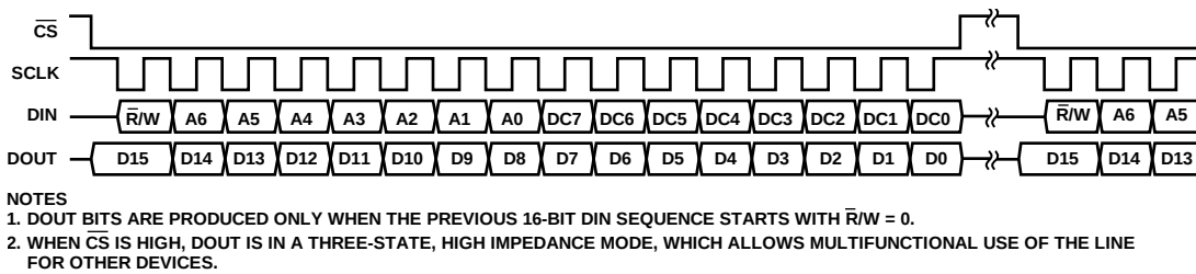
Figure 13. SPI Communication Bit Sequence
