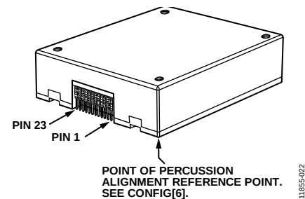
Figure 24. Point of Percussion Reference Point
