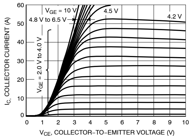
Figure 6. On-Region Characteristics @ T_J = -40^\circ\text{C}
