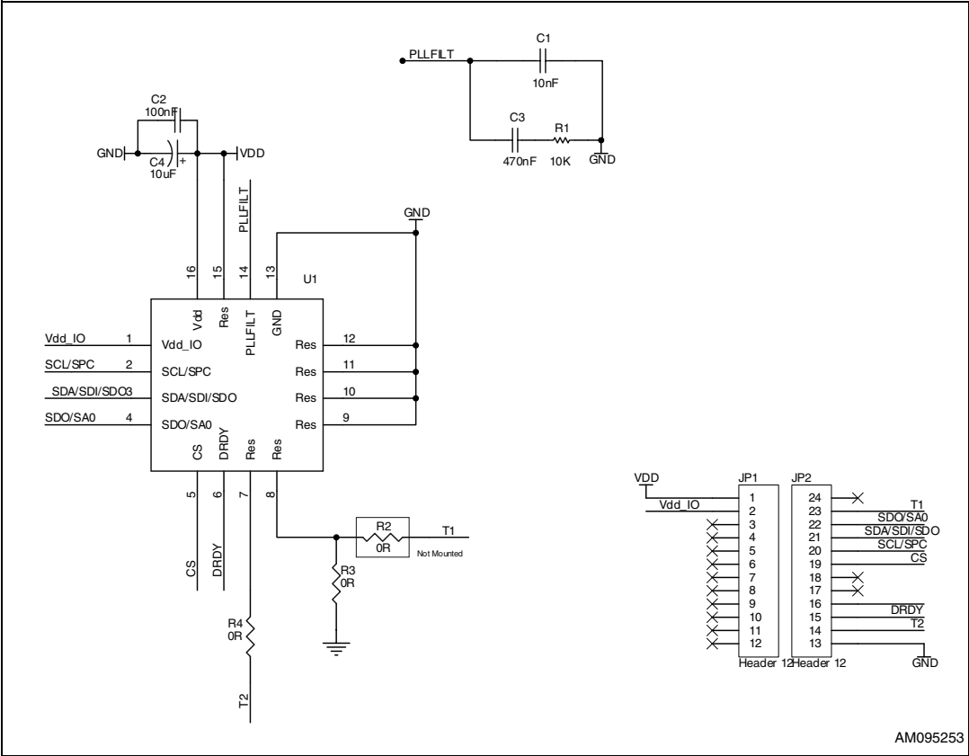
Figure 1. Circuit schematic
