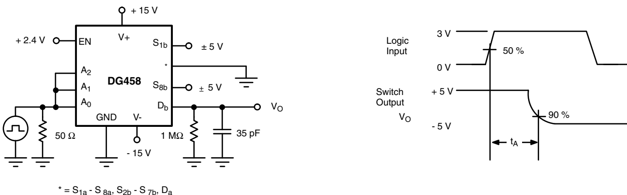
Figure 3. Transition Time
