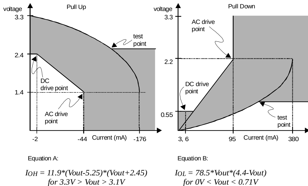
Figure 1. AC Characteristics
