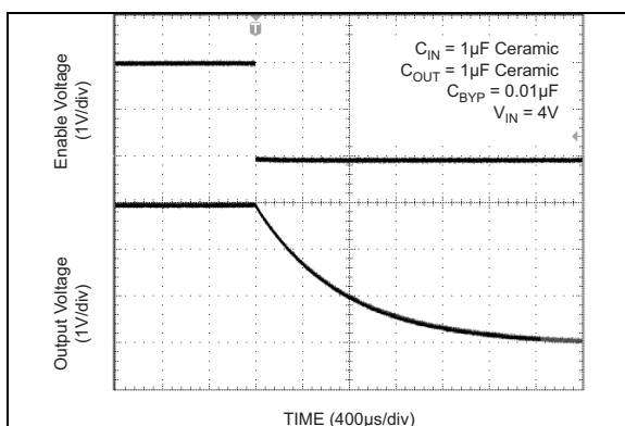
FIGURE 2-20: Shutdown Delay.
