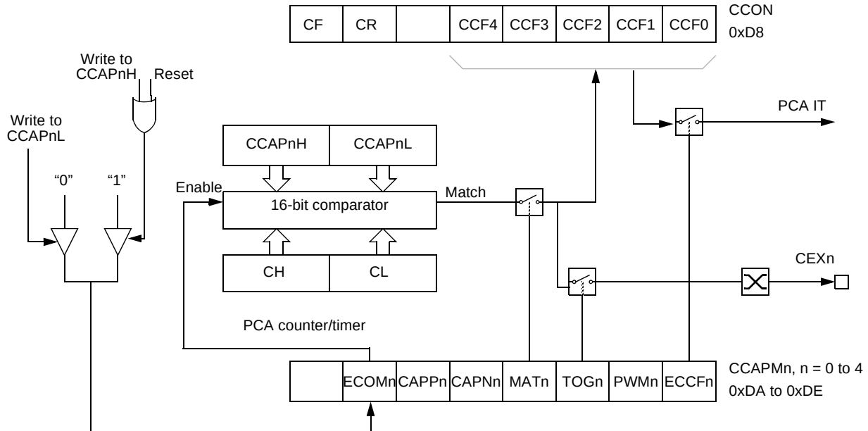
Figure 57. PCA High Speed Output Mode
