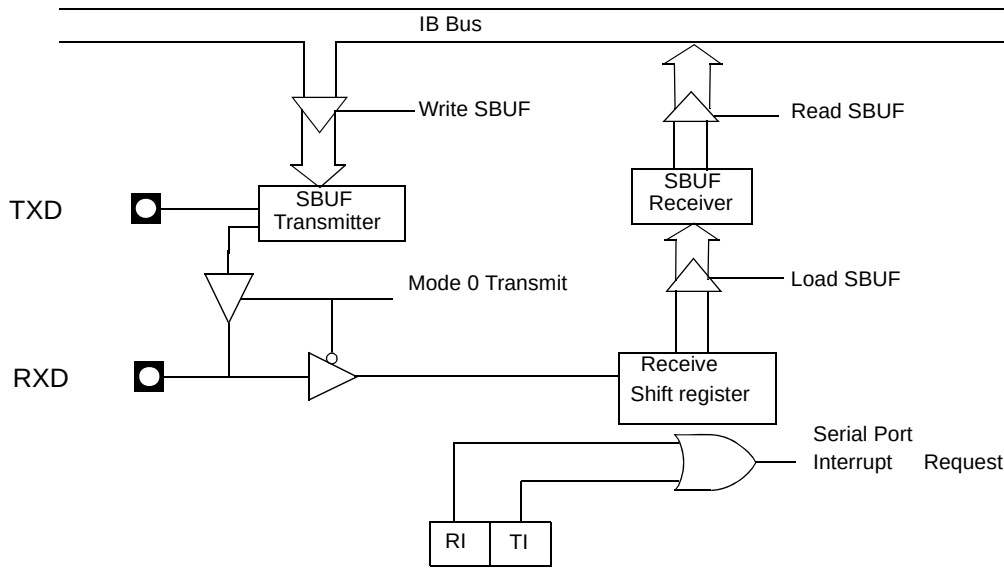
Figure 27. Serial I/O Port Block Diagram
