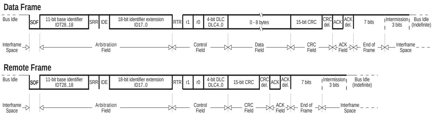
Figure 40. CAN Extended Frames
