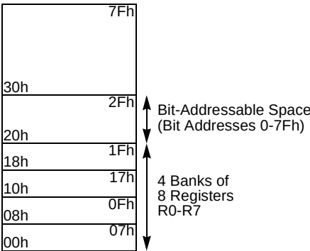
Figure 12. Lower 128 Bytes Internal RAM Organization
