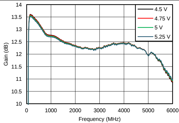
Figure 3. Gain vs Frequency V CC curves Temp = 25°C Pin = -10 dBm
