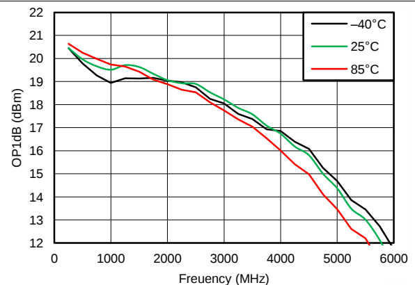
Figure 6. OP1dB vs Frequency Temp curves V CC = 5 V
