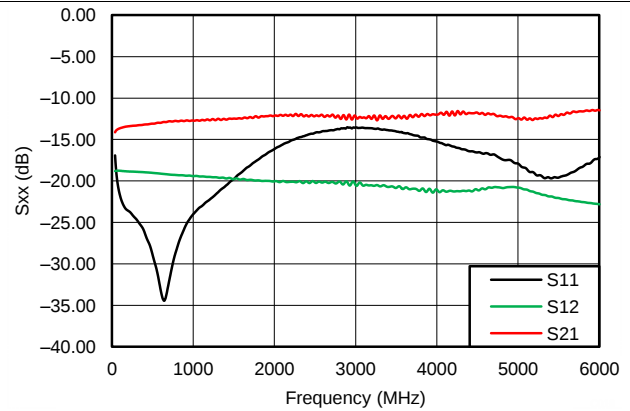
Figure 2. S11, S12, S21 V CC = 5 V Temp = 25°C 40 MHz to 6 GHz Data Taken with EVM and Bias T, De-embedded to DUT pin
