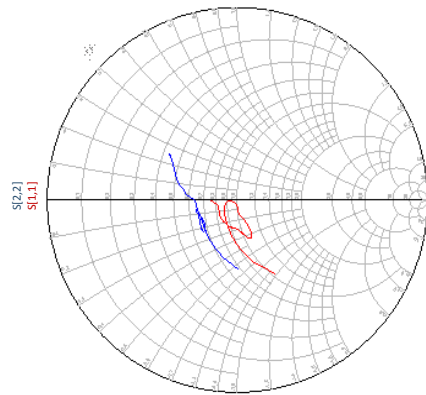
Figure 1. Smith Chart – S11, S22 V CC = 5 V Temp = 25°C 10 MHz to 6 GHz Data Taken with EVM and Bias T, De-embedded to DUT pin
