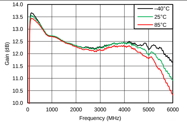
Figure 4. Gain vs Frequency Temp curves V CC = 5 V Pin = -10 dBm
