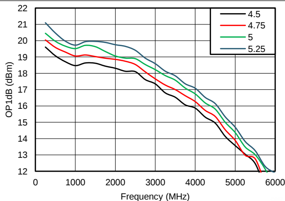
Figure 5. OP1dB vs Frequency V CC curves Temp = 25°C
