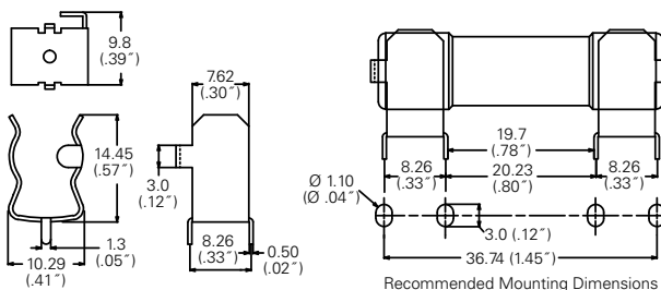
106 001 Device Dimensions
