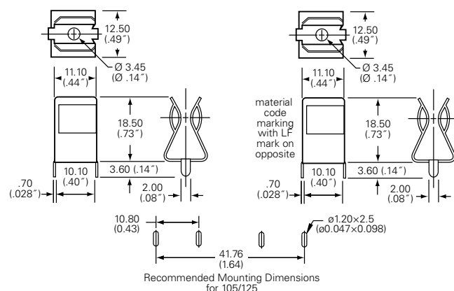
105 003 Device Dimensions
