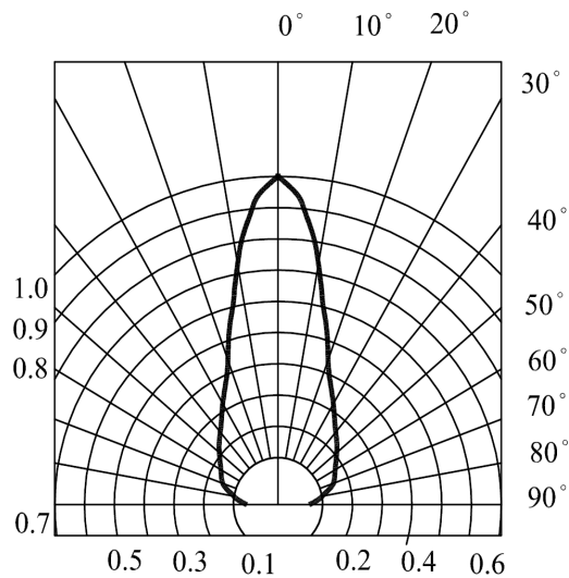
RADIATION DIAGRAM
