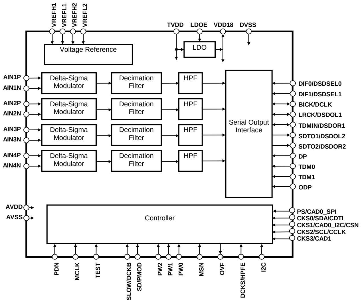
Figure 1. Block Diagram
