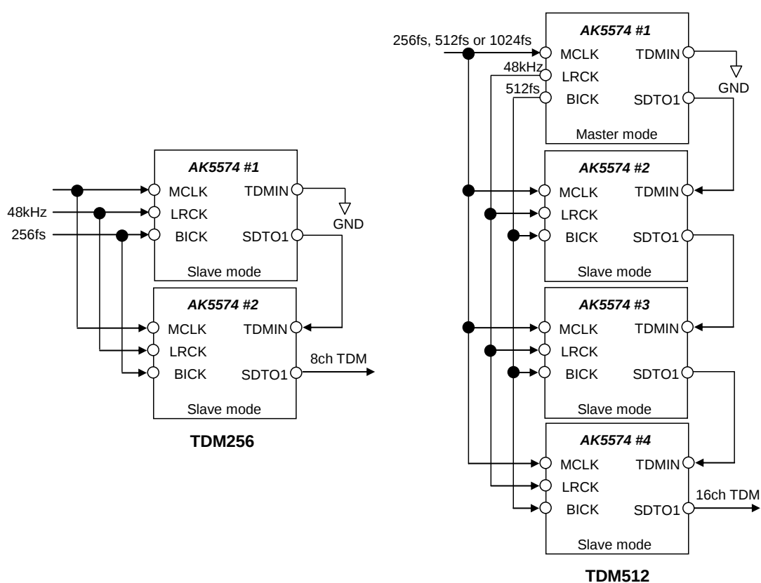
Figure 29. Cascade Connection
