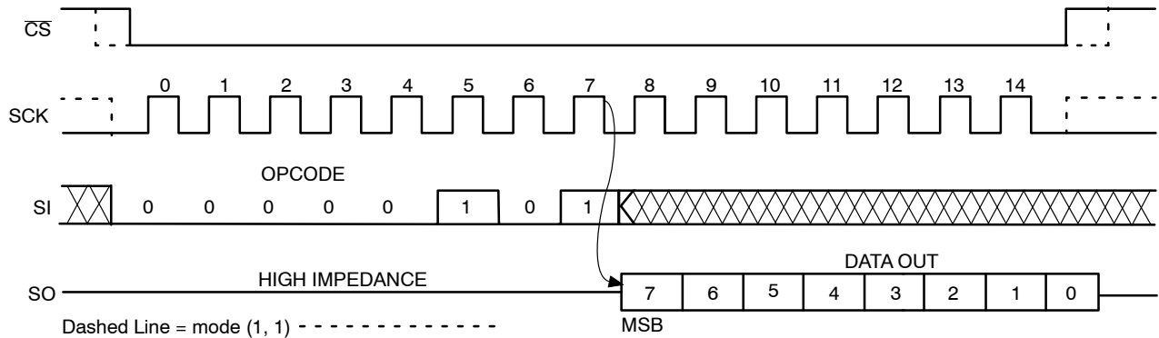
Figure 10. RDSR Timing
