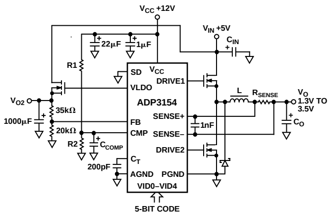
Figure 1. Typical Application
