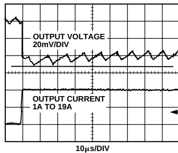
Figure 10. Load Transient Response, 1A-19A of Figure 2 Circuit
