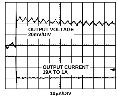
Figure 9. Load Transient Response, 19A-1A of Figure 2 Circuit
